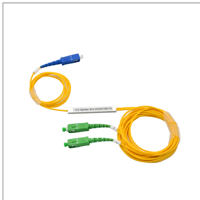
SC/APC 1x2 Steel Tube PLC Splitter 2.0mm
