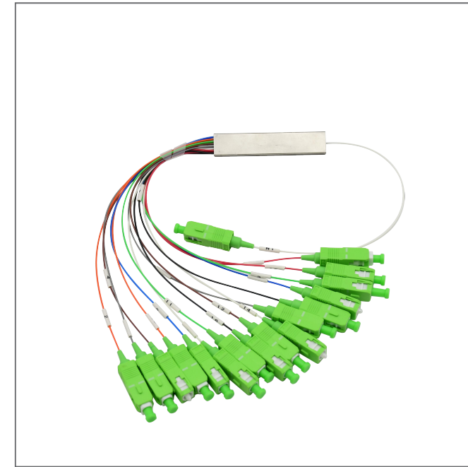
SC/APC 1x16 Steel Tube PLC Splitter 0.9mm
