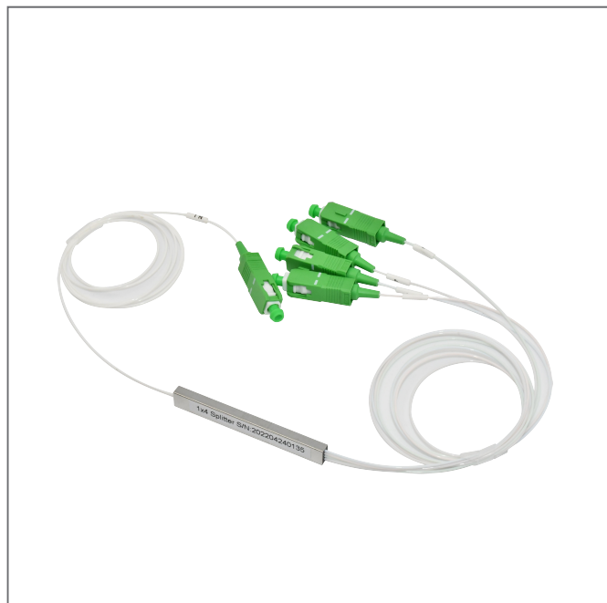
SC/APC 1x4 Steel Tube PLC Splitter 0.9mm
