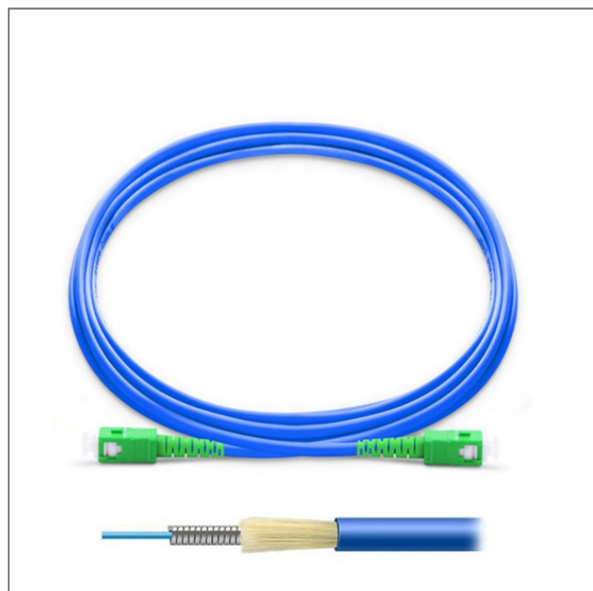
SC/APC-SC/APC Armored Simplex OS2
