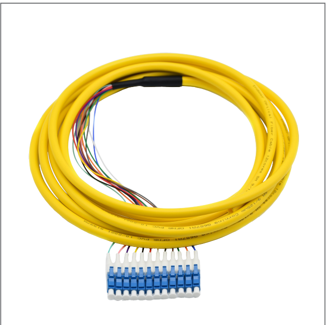
12cores LC/UPC Breakout Fiber Optic Pigtail OS2
